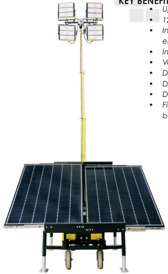
Man-portable four-wheeled cart LE978LEDVSOLAR-T4
